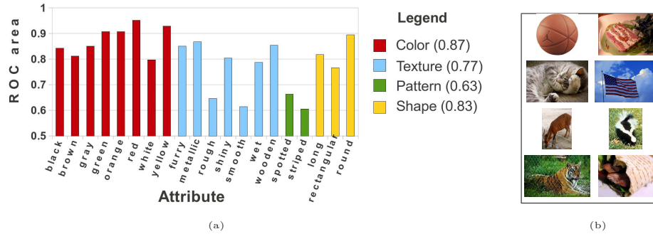
Fig. 3. (a) Performance of attribute classifiers (as measured by the area under the ROC curve) sorted by attribute type. The average performance of each type is reported in parentheses. (b) Some example images labeled by the human subjects as “striped.” This shows the difficulty of learning a good “striped” classifier on this dataset.
